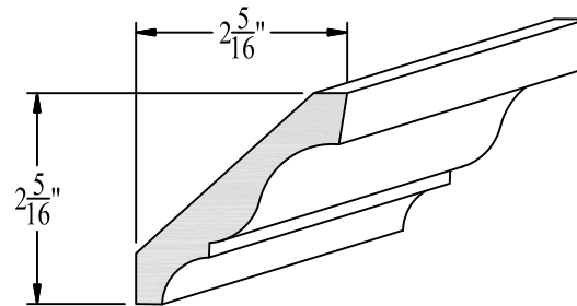
3-1/4" CROWN MOLDING AVAILABLE IN #2 CYPRESS, SELECT CYPRESS, #2 PONDEROSA PINE, #3 INLAND RED CEDAR, E-PECK™ CYPRESS, E-PECK™ PINE & E-PECK™ CEDAR
