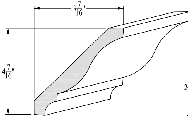
5-5/8" CROWN MOLDING AVAILABLE IN #2 CYPRESS, SELECT CYPRESS & E-PECK™ CYPRESS
