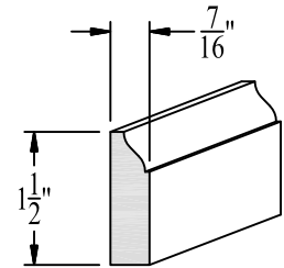
1-1/2" CEILING TRIM MOLDING AVAILABLE IN #2 CYPRESS, SELECT CYPRESS, #2 PONDEROSA PINE & #3 INLAND RED CEDAR
