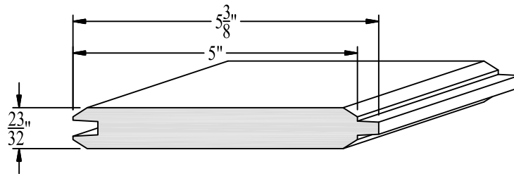
6" T&G PROFILE AVAILABLE IN #2 CYPRESS, SELECT CYPRESS, #2 PONDEROSA PINE, #3 INLAND RED CEDAR, E-PECK™ CYPRESS, E-PECK™ PINE & E-PECK™ CEDAR
